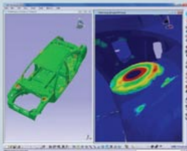
From simple safety factor analysis to detailed multi-axial fatigue.
