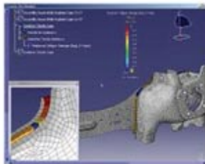
LMS Virtual.Lab Durability Seam Weld supports accurate and efficient simulation of seam welds.
